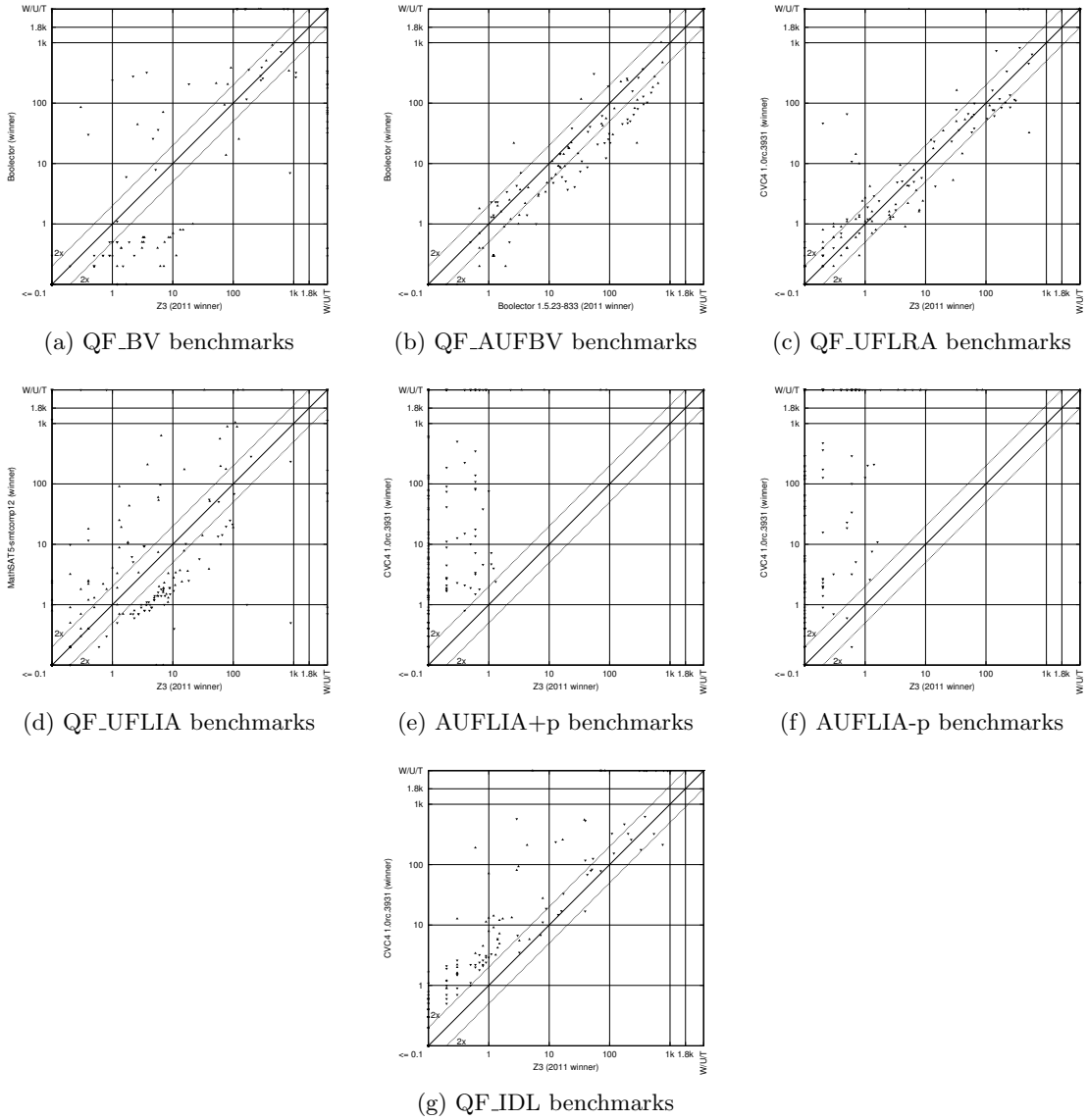
Figure 2: Comparisons of 2012 and 2011 winners the main track divisions. The axes show time taken, so marks below and to the right of the diagonals show improvement in 2012.
