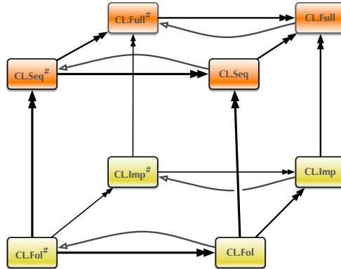
Figure 2: Elimination of the module construct in CL
