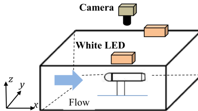
Fig. 1. Experimental setup for skin-friction measurement
