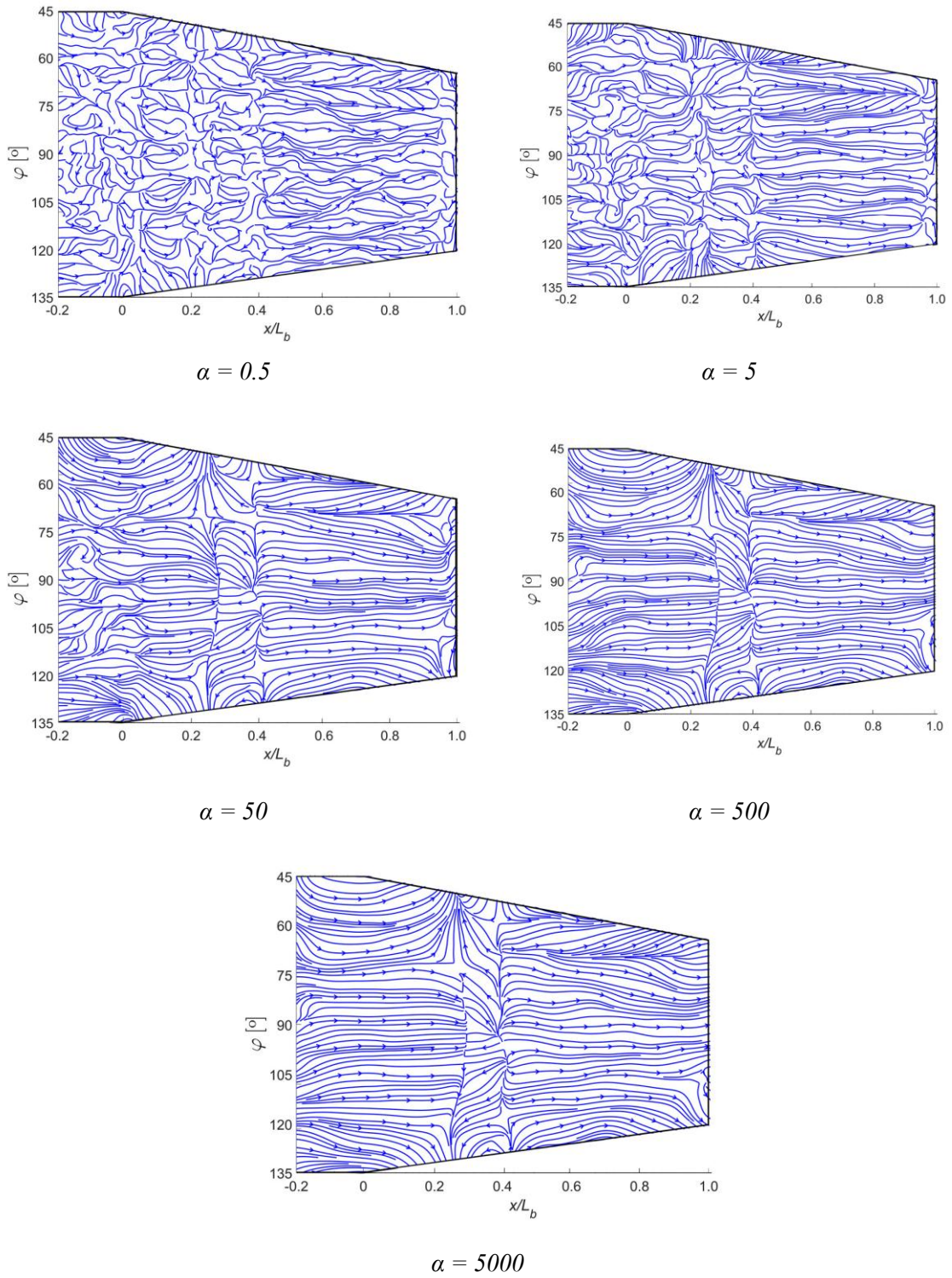
Fig. 4. Skin-friction fields for different Lagrange multiples.
