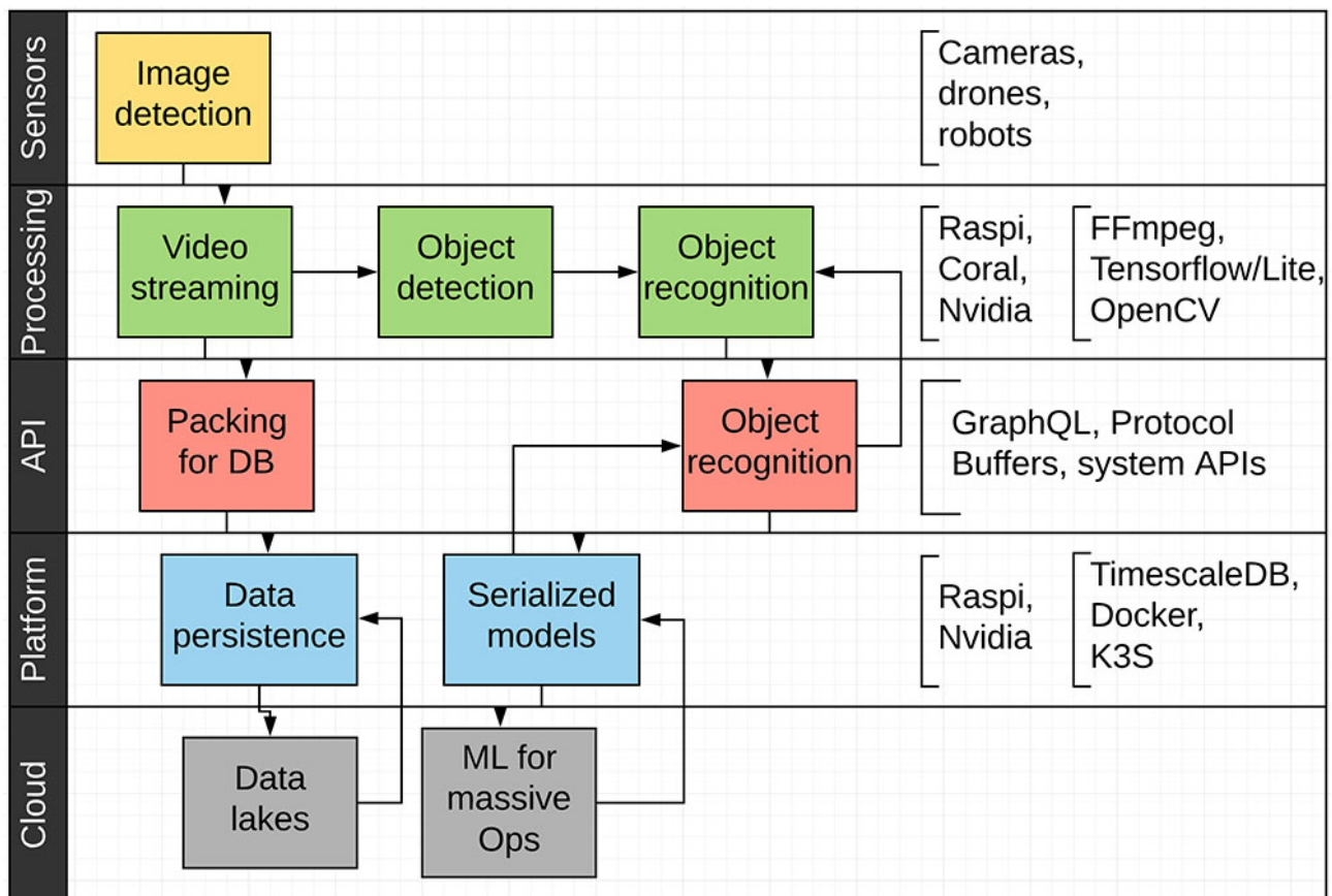
Fig. 2. Image detection and respective ML process with participating devices and software tools.
