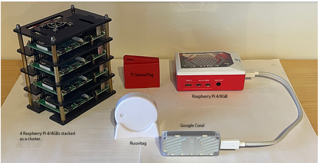
Fig. 1. Example edge system components.
