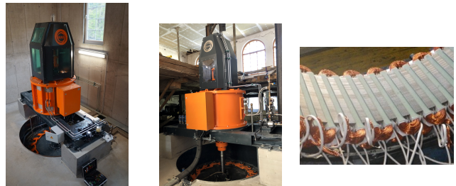
Fig. 2. Hydropower generator with corresponding coil winding
