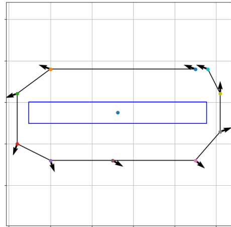
Fig. 5. Planned points for the winding process
