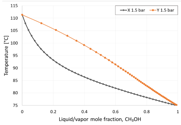
Figure 2. Txy diagram for methanol/water
