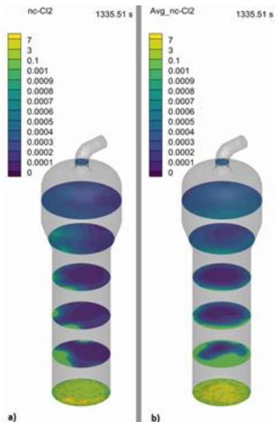
Figure 7. \text{Cl}_2 concentration ( \text{mole/m}^3 ) in different heights, a) \text{Cl}_2 concentration at the specific time, and b) Average \text{Cl}_2 concentration in the last 300 seconds.
