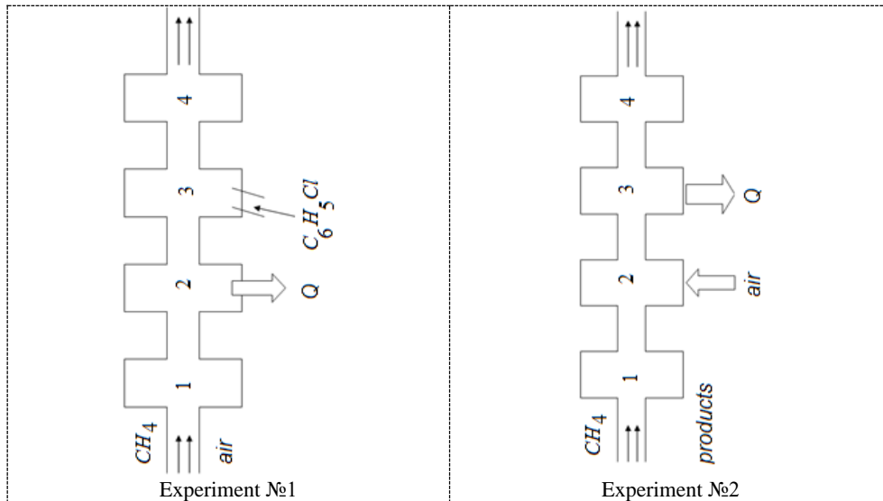
Fig. 1 The scheme of a mathematical model for carrying out a numerical experiment: 1, 2, 3, 4 - flowing non-stationary reactors
