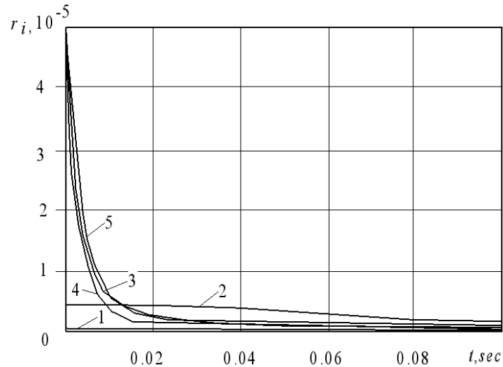
Fig. 5 Change of a mole dole atomic hydrogen H at a mass fraction of chlorobenzene g=0.0001 from composition of mixture and various reference temperatures: 1- 1000 K; 2- 1100 K; 3- 1200 K; 4- 1300 K; 5- 1400 K
