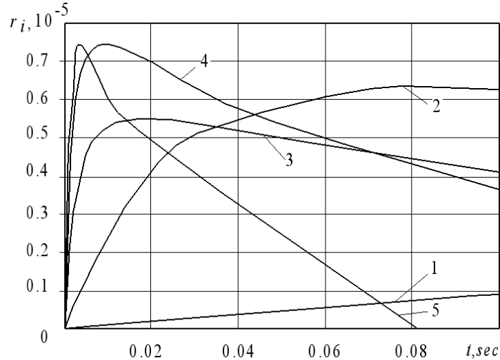
Fig. 3 Change of a mole dole dichlorobenzene at a mass fraction of chlorobenzene g=0.0001 from composition of mixture and various reference temperatures: 1- 1000 K; 2- 1100 K; 3- 1200 K; 4- 1300 K; 5- 1400 K
