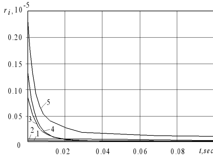
Fig. 6 Change of a mole dole OH at a mass fraction of chlorobenzene g=0.0001 from composition of mixture and various reference temperatures: 1- 1000 K; 2- 1100 K; 3- 1200 K; 4- 1300 K; 5- 1400 K
