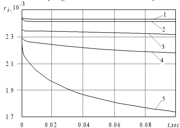
Fig. 2 Change of a mole dose of chlorobenzene at a mass fraction g=0.01 from composition of mixture and various reference temperatures: 1- 1000 K; 2- 1100 K; 3- 1200 K; 4- 1300 K; 5- 1400 K
