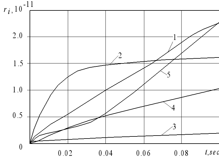
Fig. 4 Change of a mole dole chloromethane CH_3Cl at a mass fraction of chlorobenzene g=0.0001 from composition of mixture and various reference temperatures: 1- 1000 K; 2- 1100 K; 3- 1200 K; 4- 1300 K; 5- 1400 K
