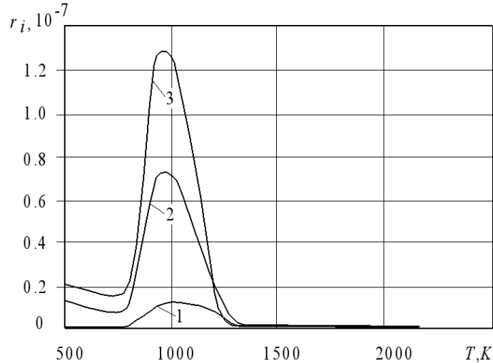
Fig. 7 Change of mole dole of chloromethane depending on temperature and a mass fraction of the brought decomposition products of chemical fuel: 1- g=0.03 ; 2- g=0.04 ; 3- g=0.05
