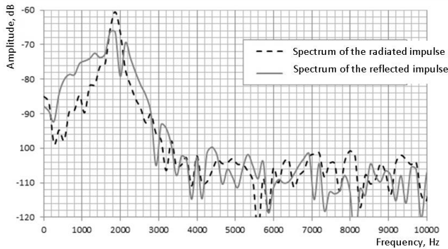
Fig. 6. The spectra of the forward and return signal
