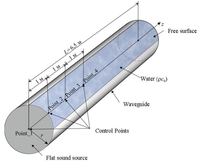
Fig. 3. Numerical model of a cylindrical waveguide
