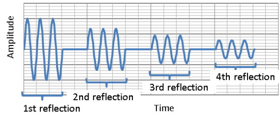
Fig. 2. Registered pulses
