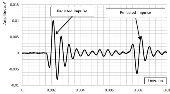
Fig. 5. Echo signal in the waveguide when a short sinusoidal pulse is applied to the piston
