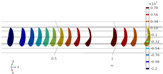
Fig. 8. The wave front (ISO surfaces of equal pressure) in a waveguide with "non- absolutely " rigid walls
