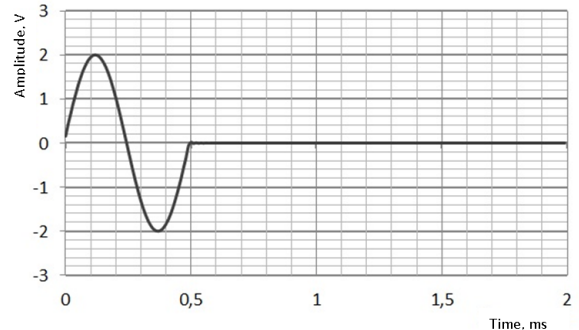
Fig. 4. A single sinusoidal pulse applied to the electrodynamic vibrator
