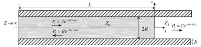
Fig. 1. A cylindrical waveguide filled with water
