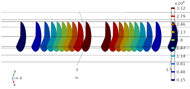
Fig. 7. The wave front (ISO surfaces of equal pressure) in a waveguide with "absolutely" rigid walls
